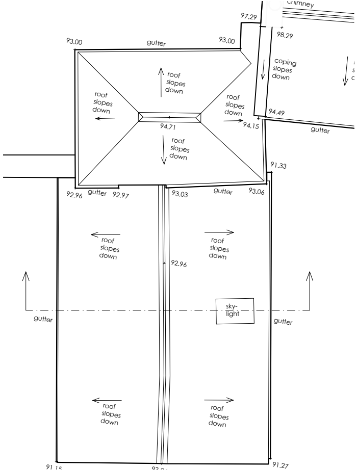
Roof Plan
