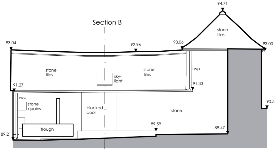
East Elevation
