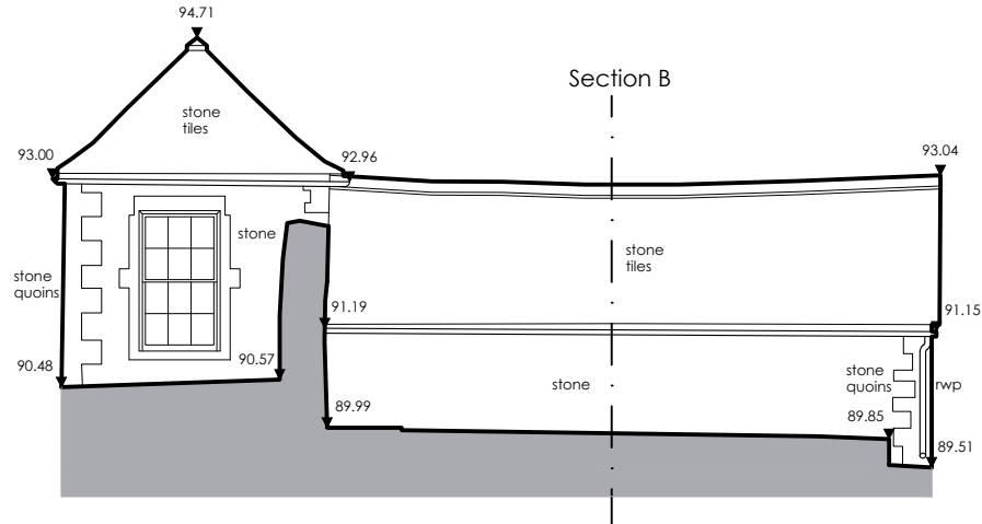
West Elevation
