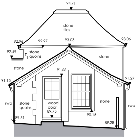
South Elevation
