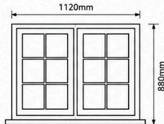
WINDOW 1 LH REAR ELEVATION
