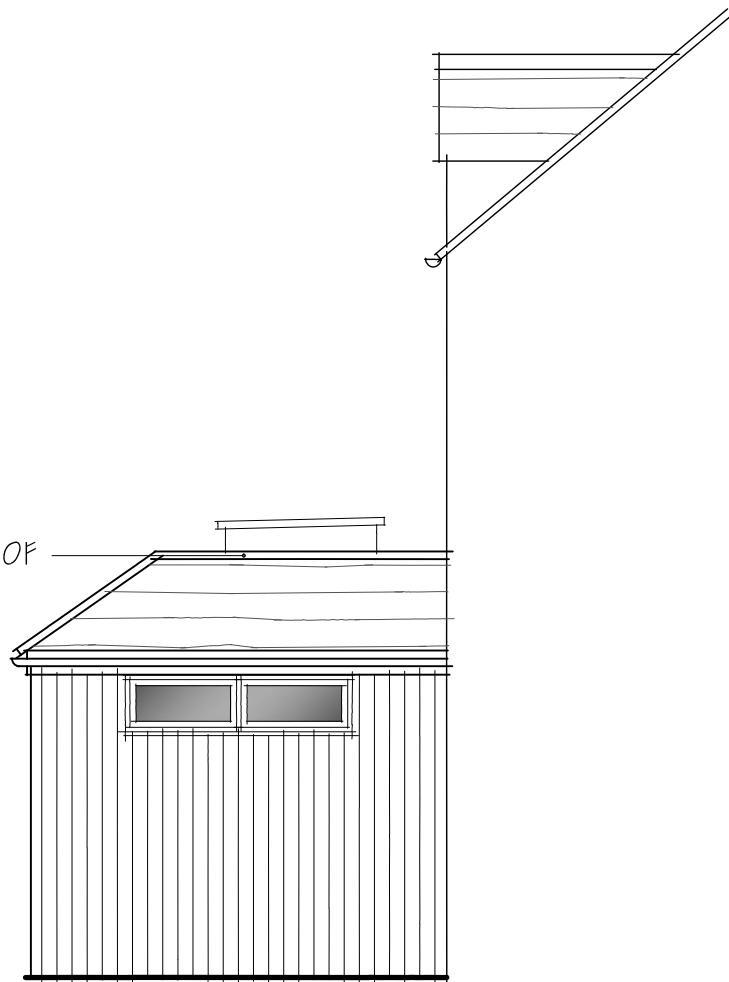
EAST ELEVATION
