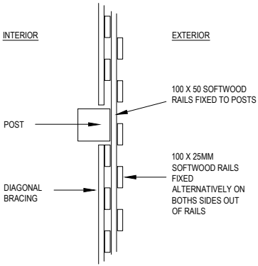
PLAN DETAIL
