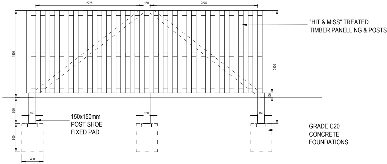
DETAILED SIDE ELEVATION OF BIN STORE
