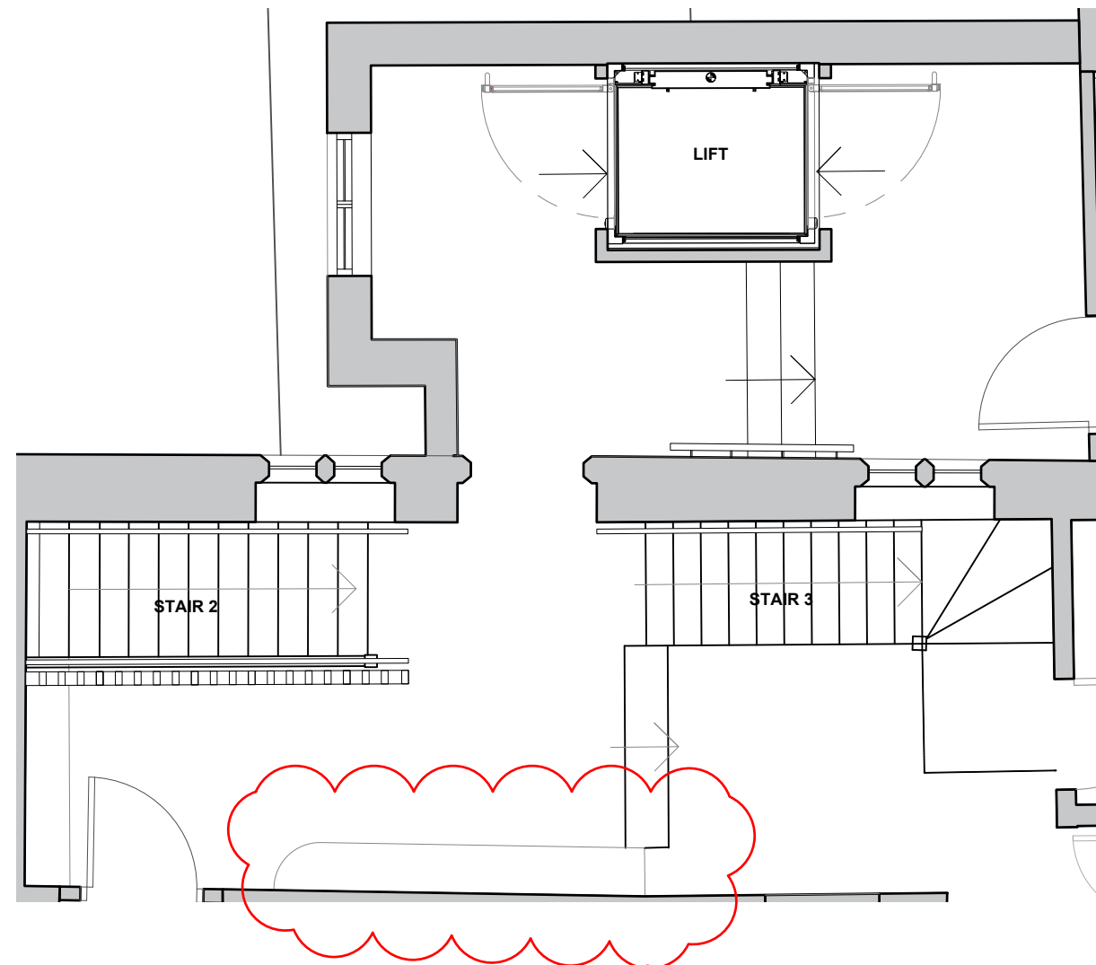
2 Existing First Floor Stair 3 Plan Scale 1:50
