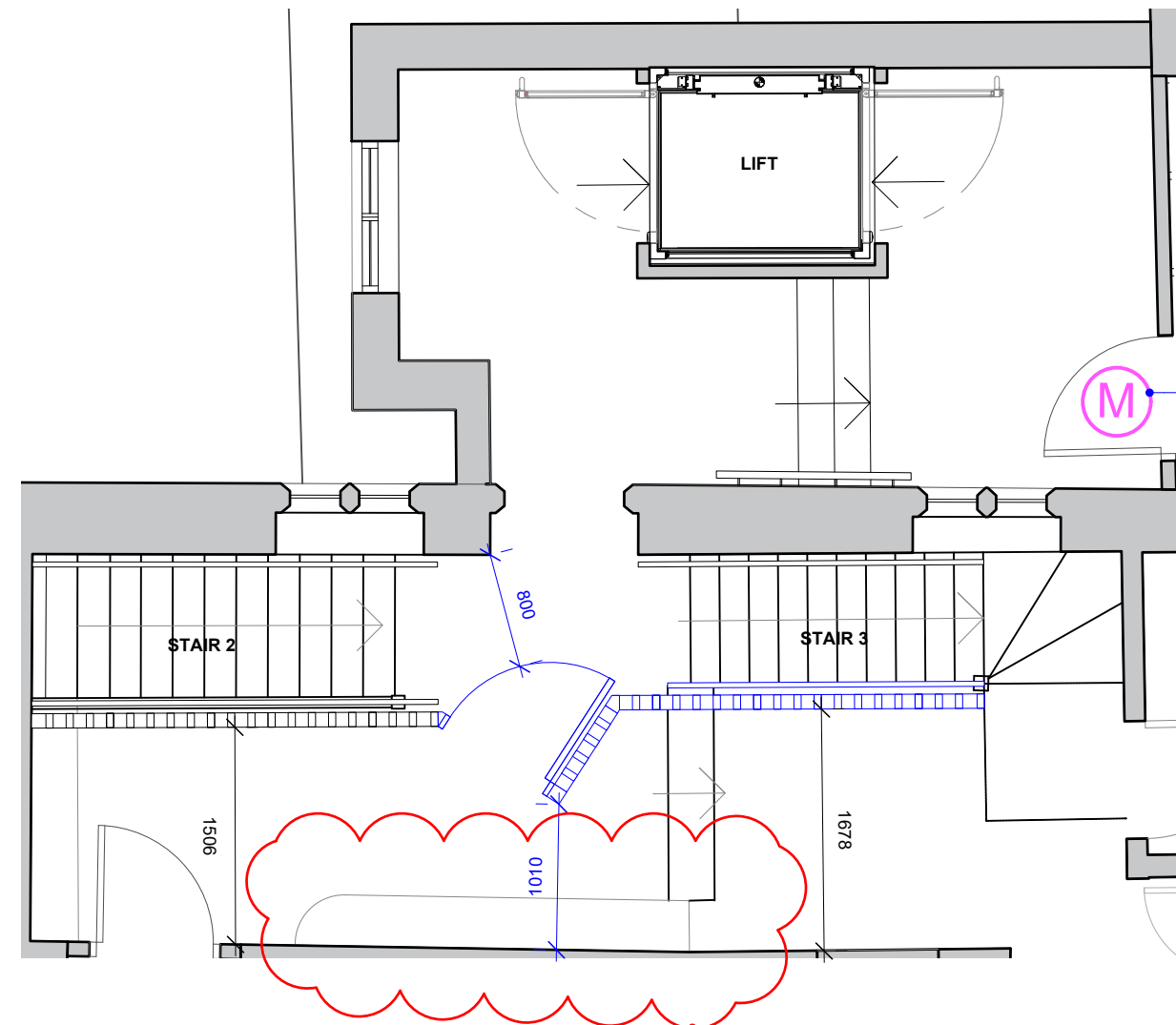
3 Proposed First Floor Stair 3 Plan Scale 1:50
