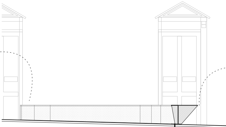
C-C SECTION DETAIL 1:50
