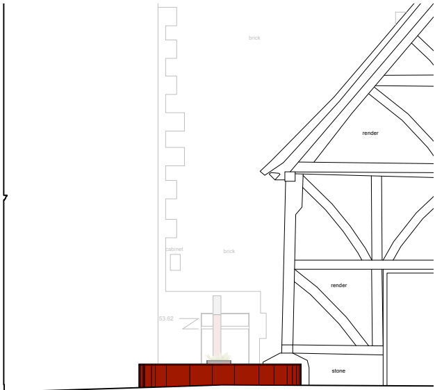
SOUTH EAST ELEVATION 1:100
