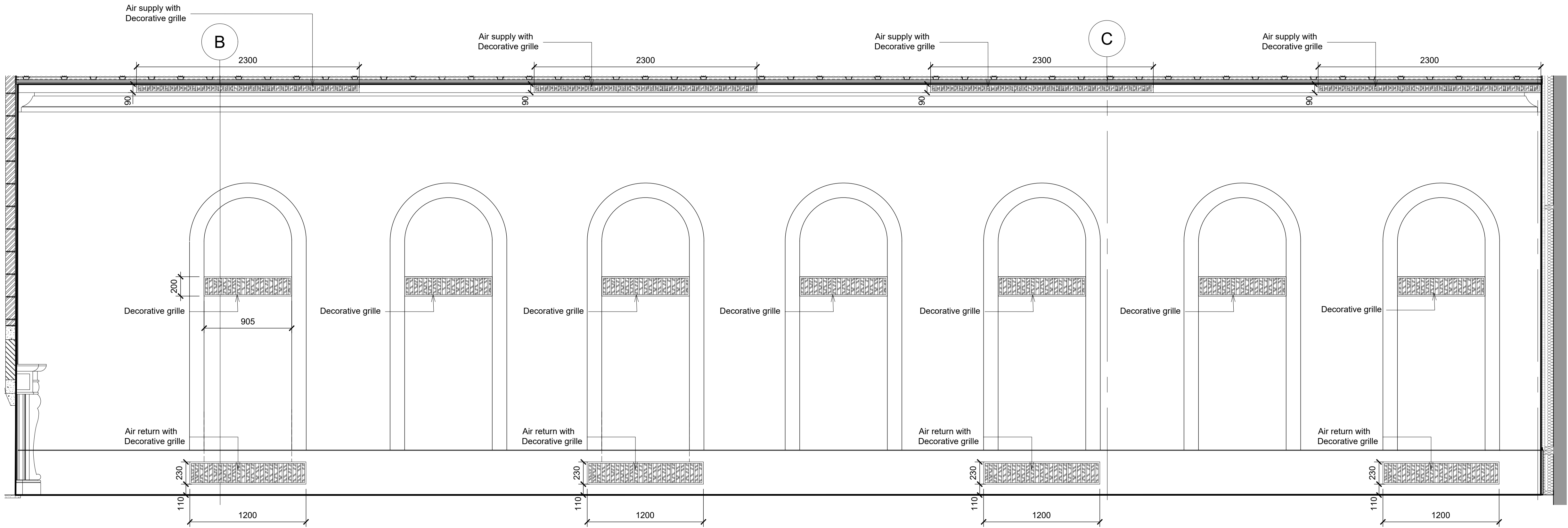
01 ELEVATION OF SITTING ROOM G24 1:25 @ A1 / 1:50 @ A3
