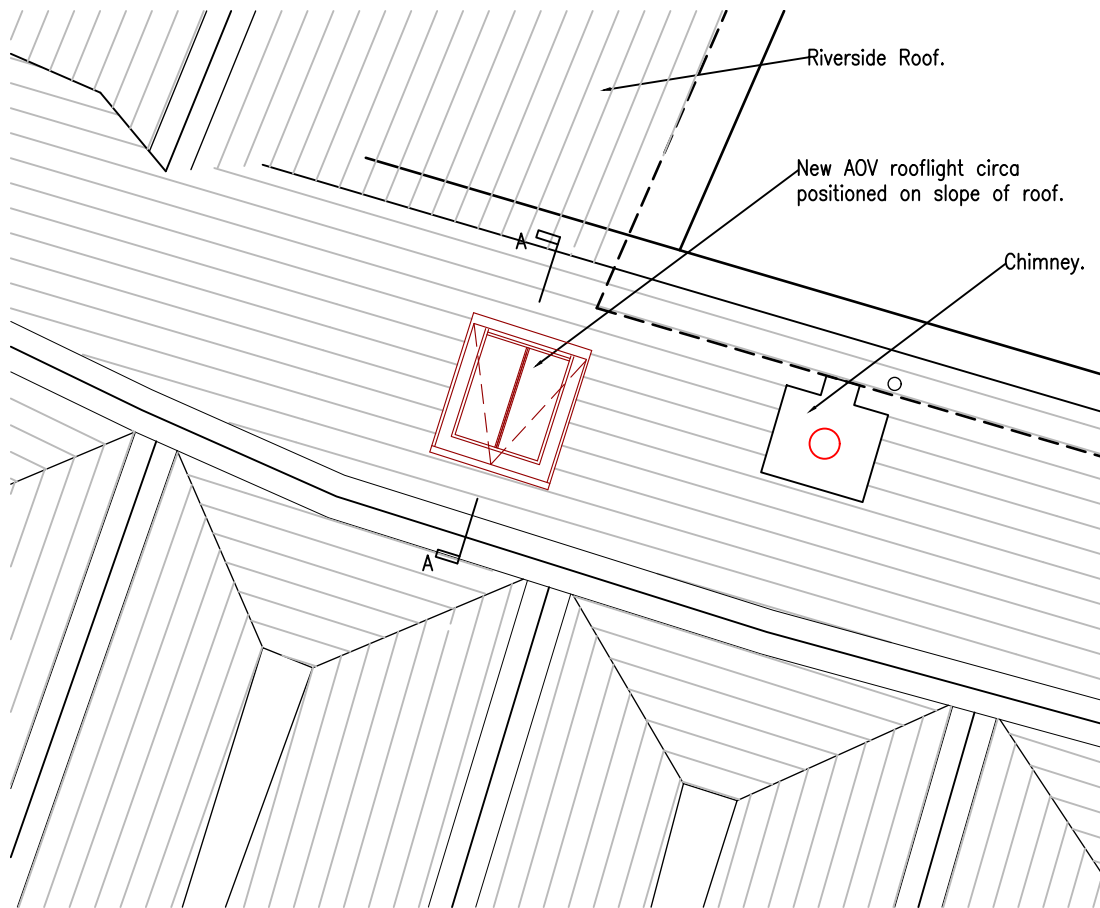
SOUTHBLOCK, ROOF PLAN, PROPOSED AOV – SCALE 1:50
