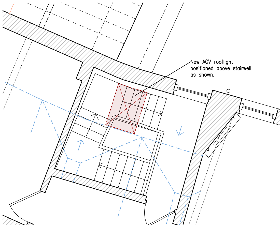
SOUTHBLOCK, SECOND FLOOR STAIRWELL – SCALE 1:50
