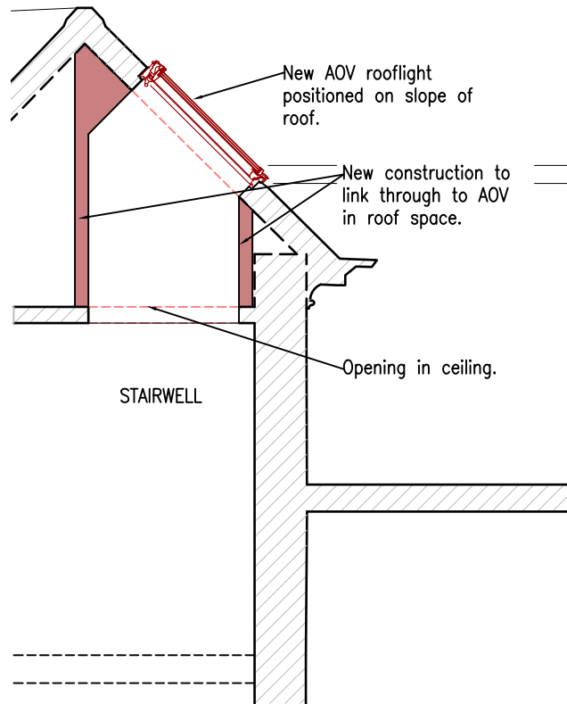
SOUTHBLOCK, SECTION AA – SCALE 1:50
