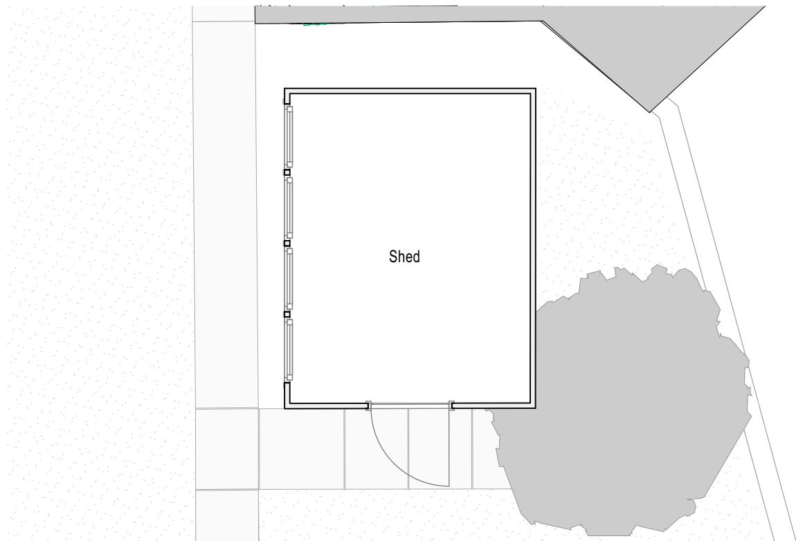
0. Existing Shed Ground Floor Plan 1:50
