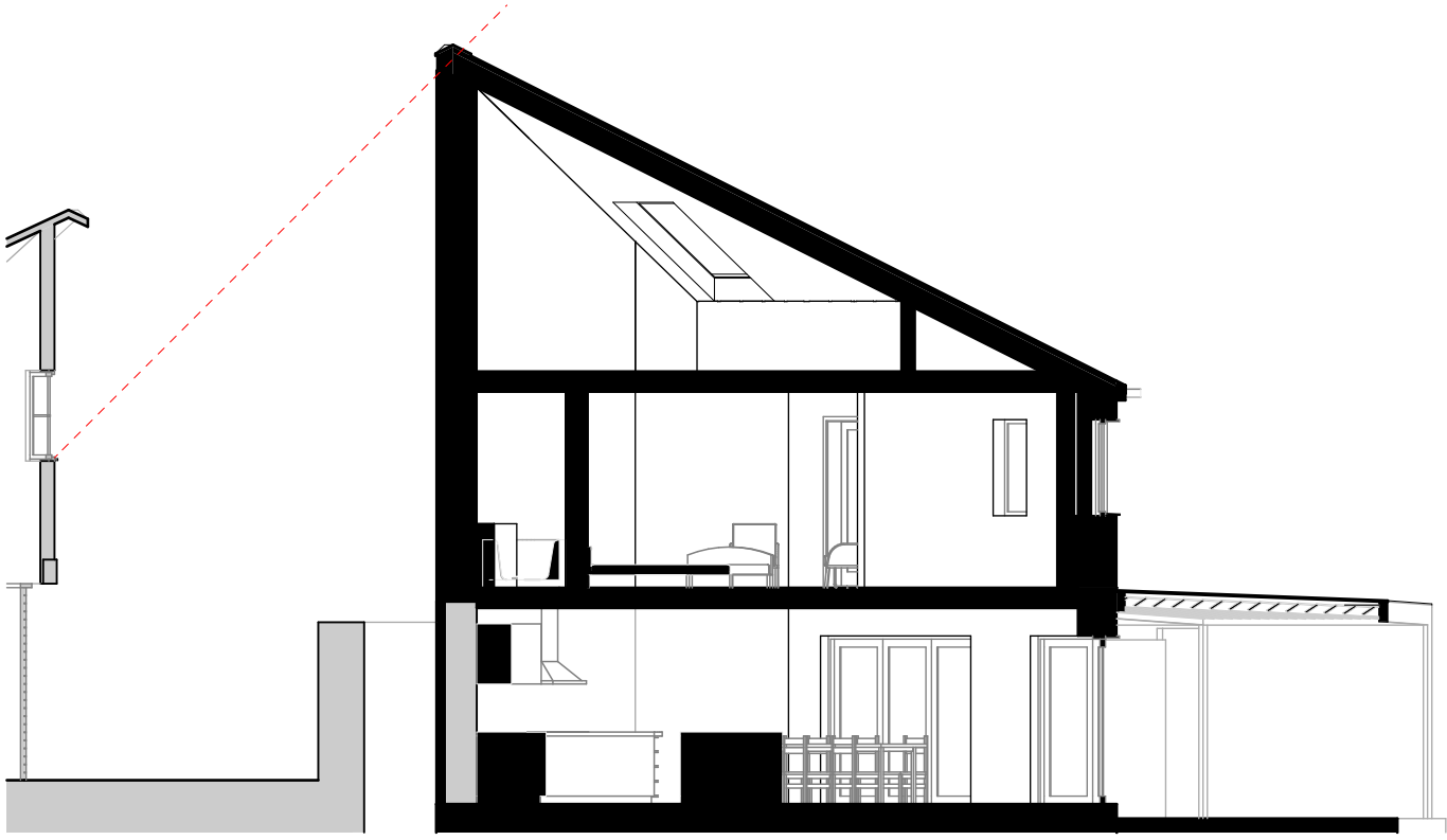
S58 Section at Autumn/Spring Equinox line 1:100
