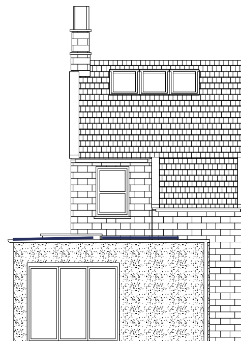
North Facing Rear Elevation
