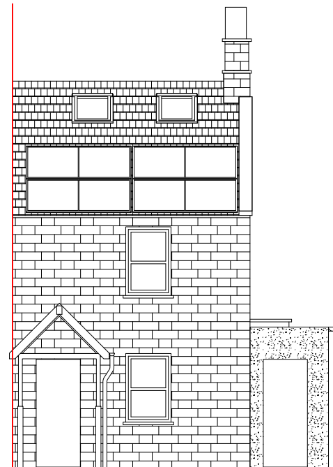
South Facing Front Elevation
