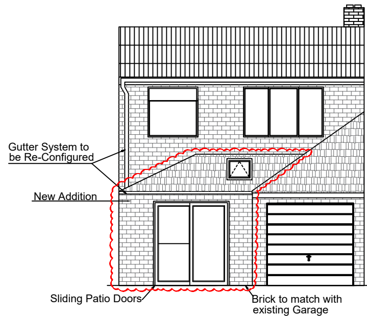
12 PROPOSED WEST ELEVATION - 1 : 100 @ A3
