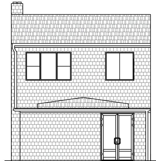
10 PROPOSED EAST ELEVATION - 1 : 100 @ A3 No development on rear side
