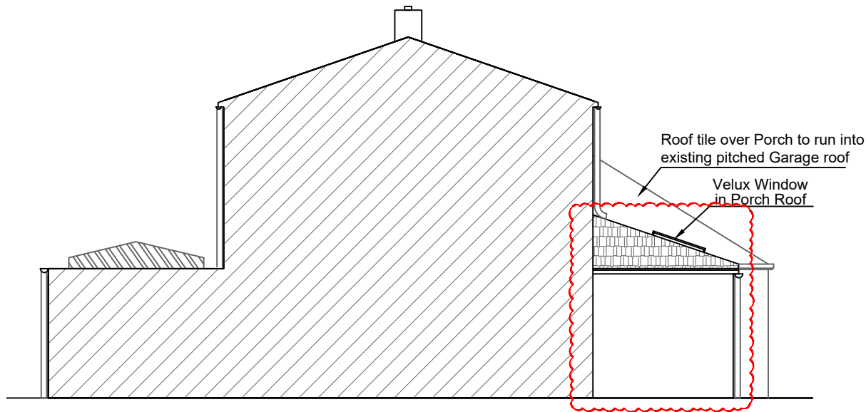
11 PROPOSED NORTH ELEVATION - 1 : 100 @ A3
