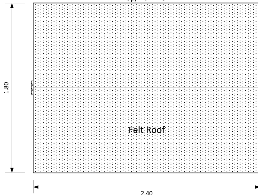
Top/Plan View
