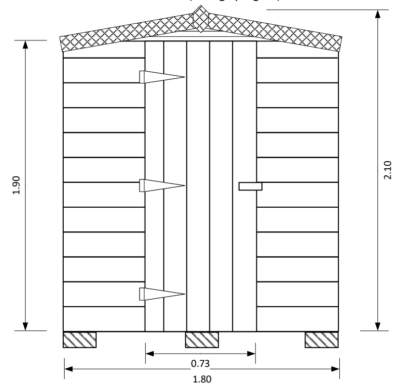
Front View (facing Lychgate)
