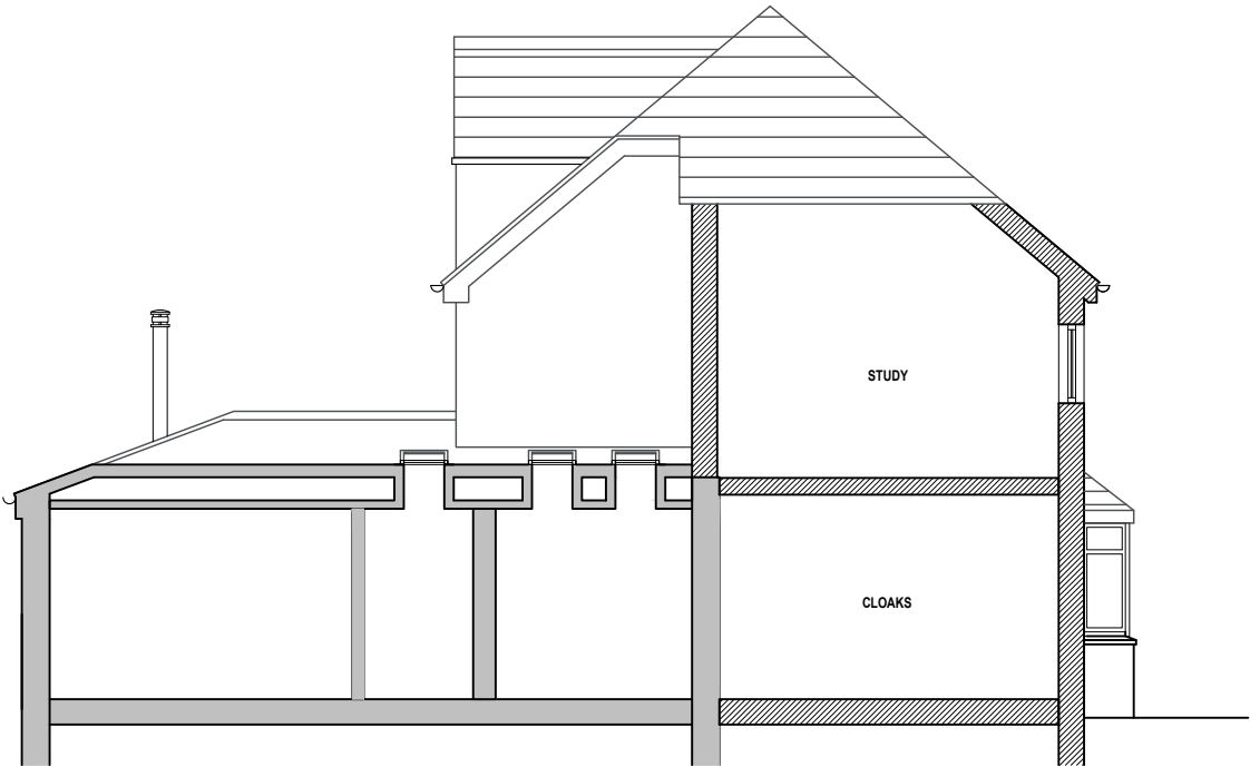
PROPOSED SECTION
