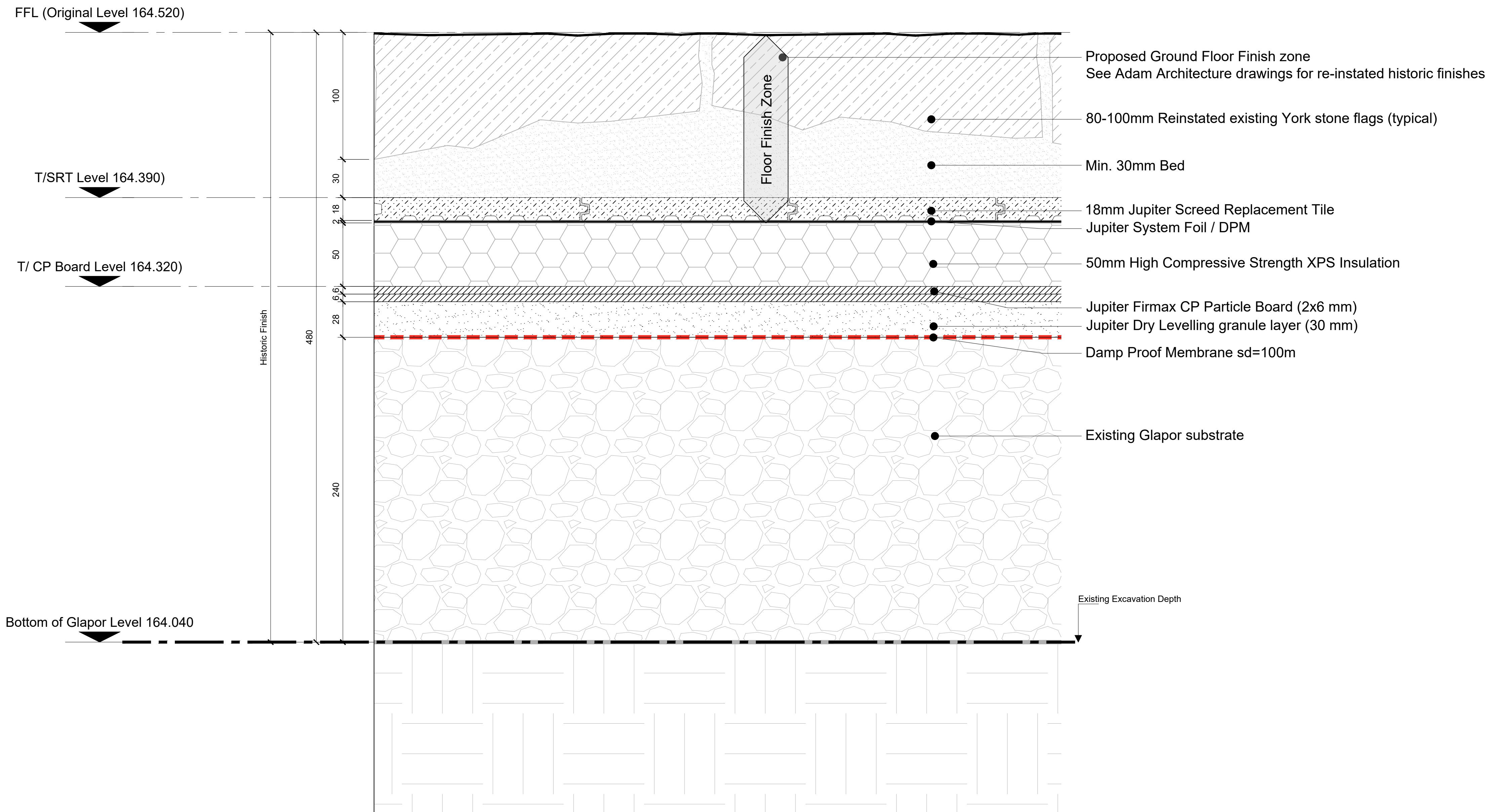
1 Ground Floor Finishes on SRT - No Overlay 1:2 @ A1 / 1:4 @ A3 - GROUND FLOOR
