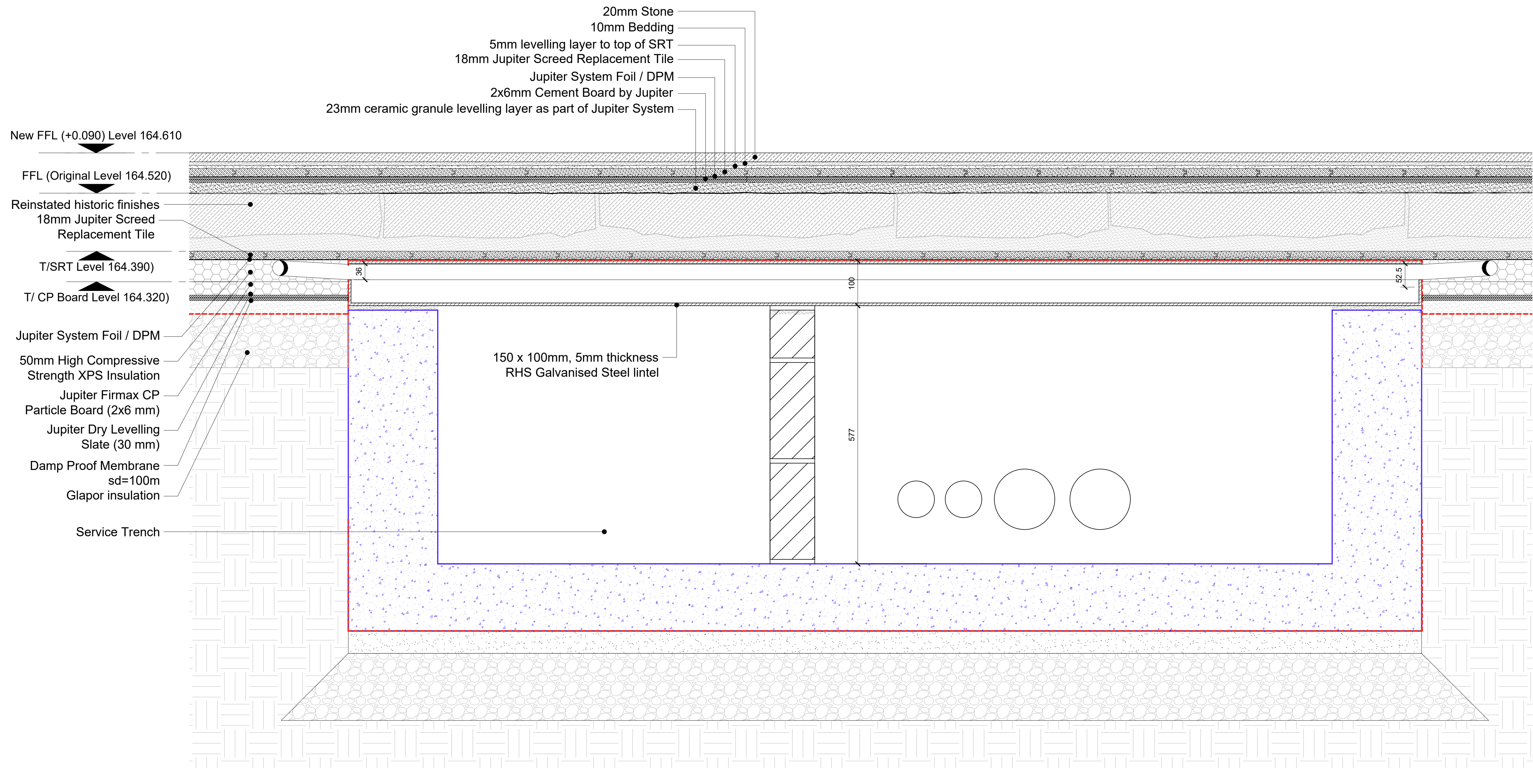
1 Section through the Trench Services 1:5 @ A1 / 1:10 @ A3 - GROUND FLOOR
