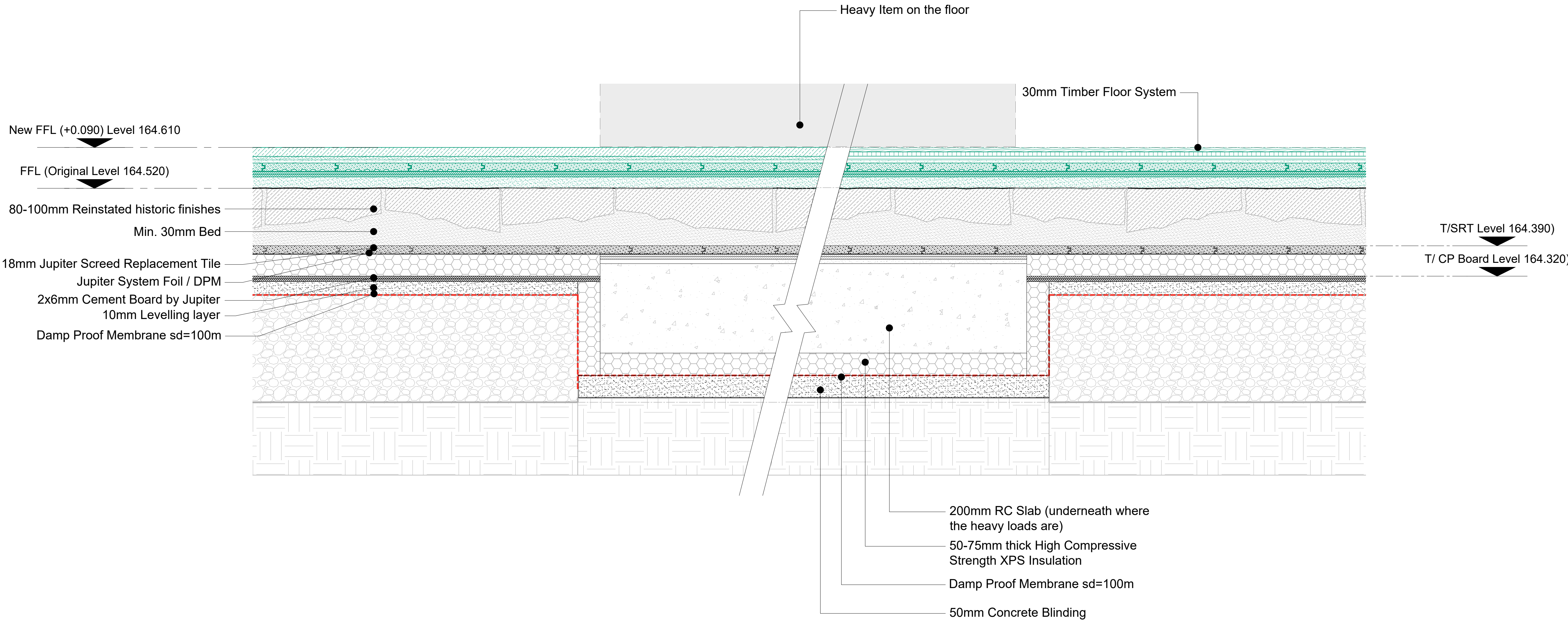
1 Section through the Heavy Loads sitting on the floor 1:5 @ A1 / 1:10 @ A3 - GROUND FLOOR
