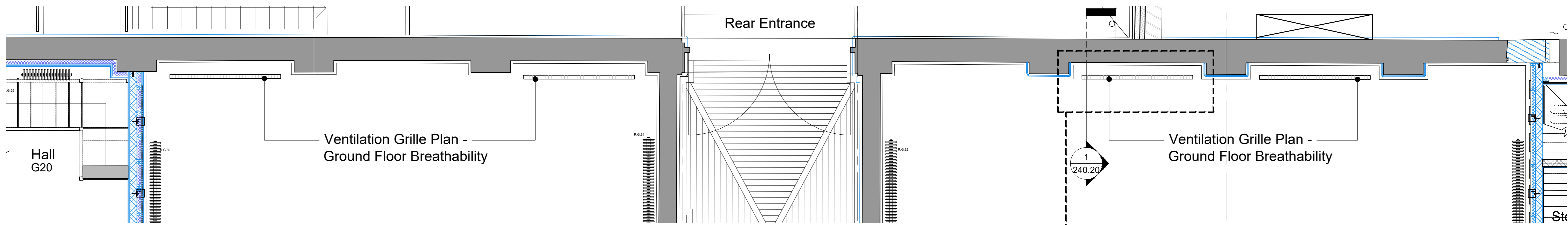
3 Ventilation Grille Plan - Ground Floor Breathability 1:50 @ A1 / 1:100 @ A3 - GROUND FLOOR
