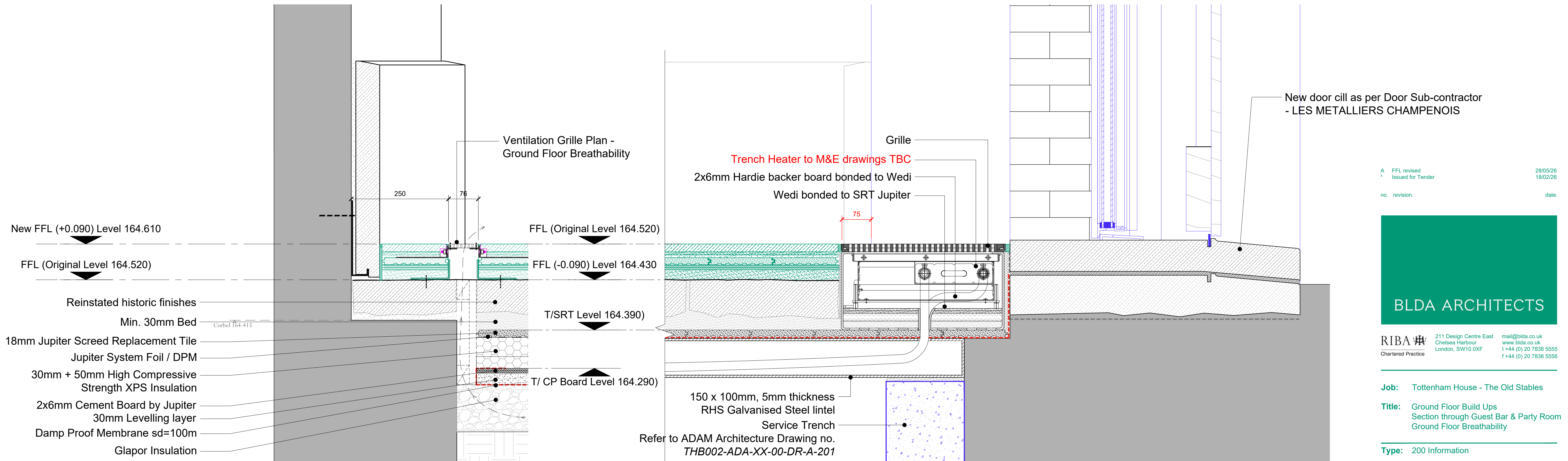
1 Section through Guest Bar & Party Room Ground Floor Breathability 1:5 @ A1 / 1:10 @ A3 - GROUND FLOOR
