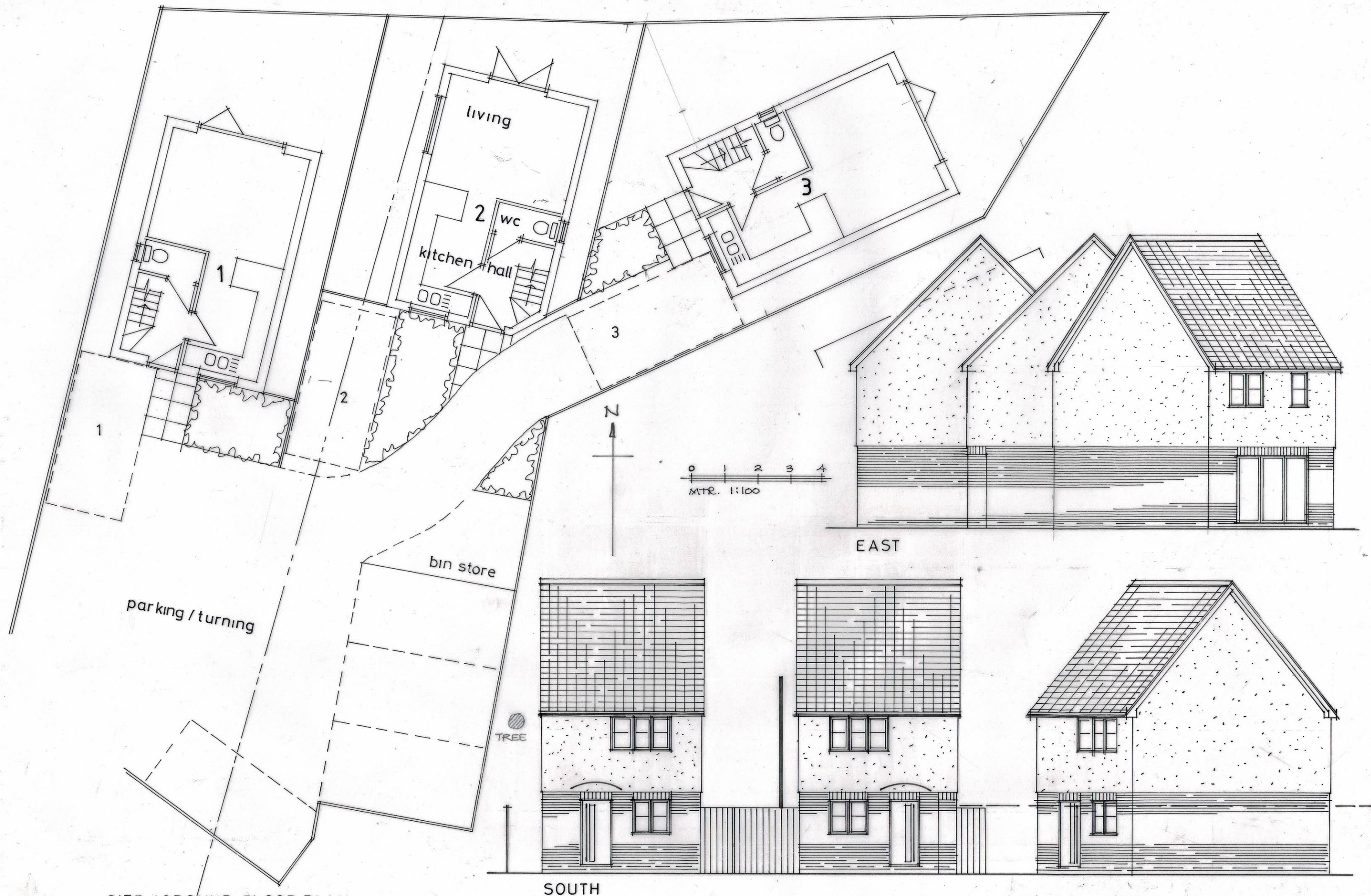
SITE / GROUND FLOOR PLAN
