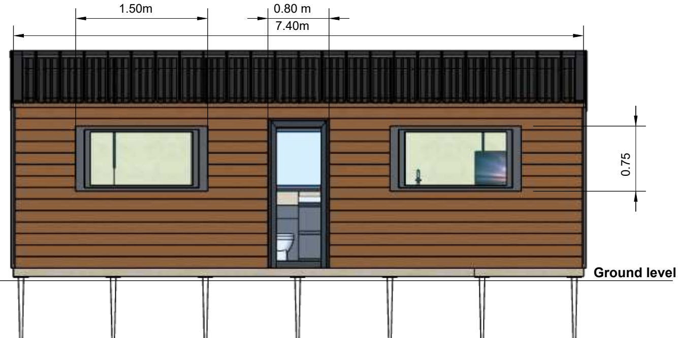
Front Elevation
