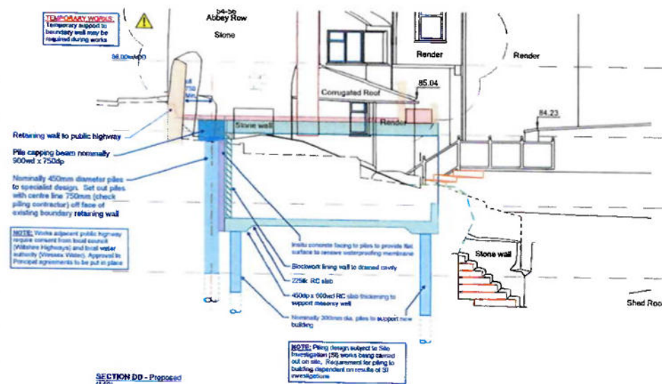
SECTION DD - Proposed (1:50)
