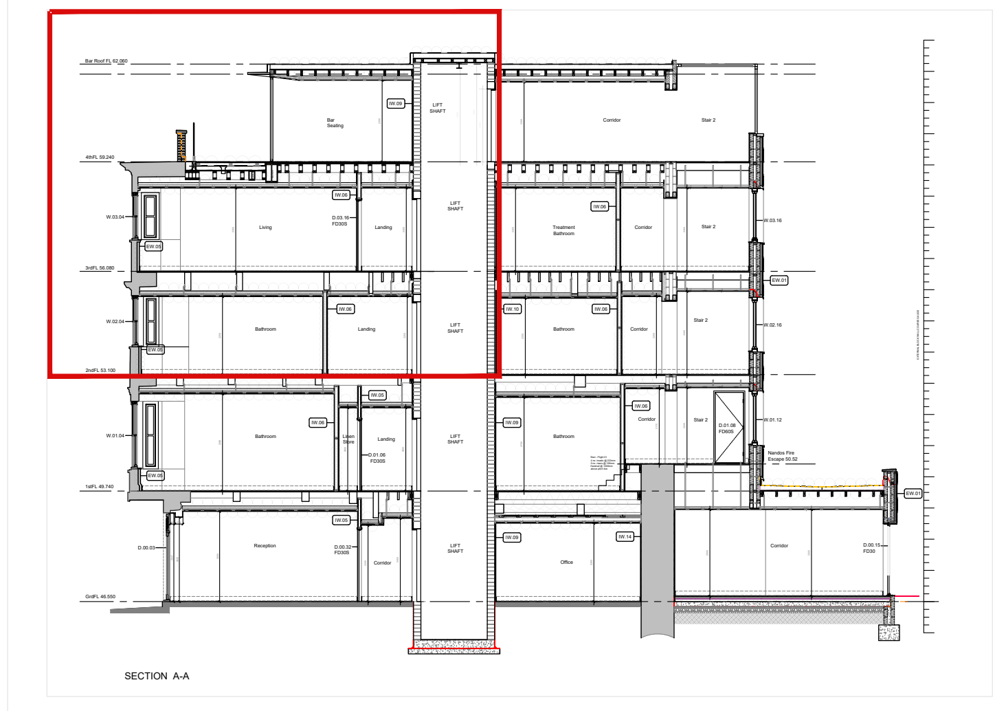
3 Section A-A - Section Key 1:150
