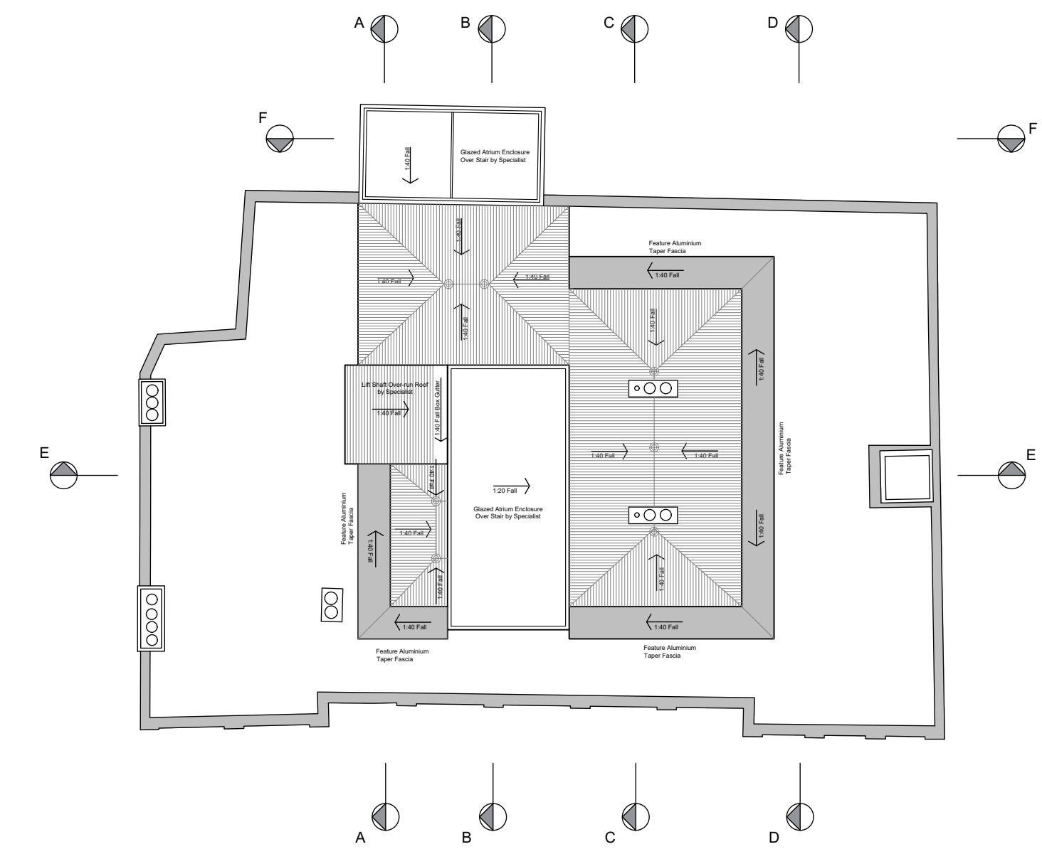
2 Fourth Floor Plan - Section key 1:150
