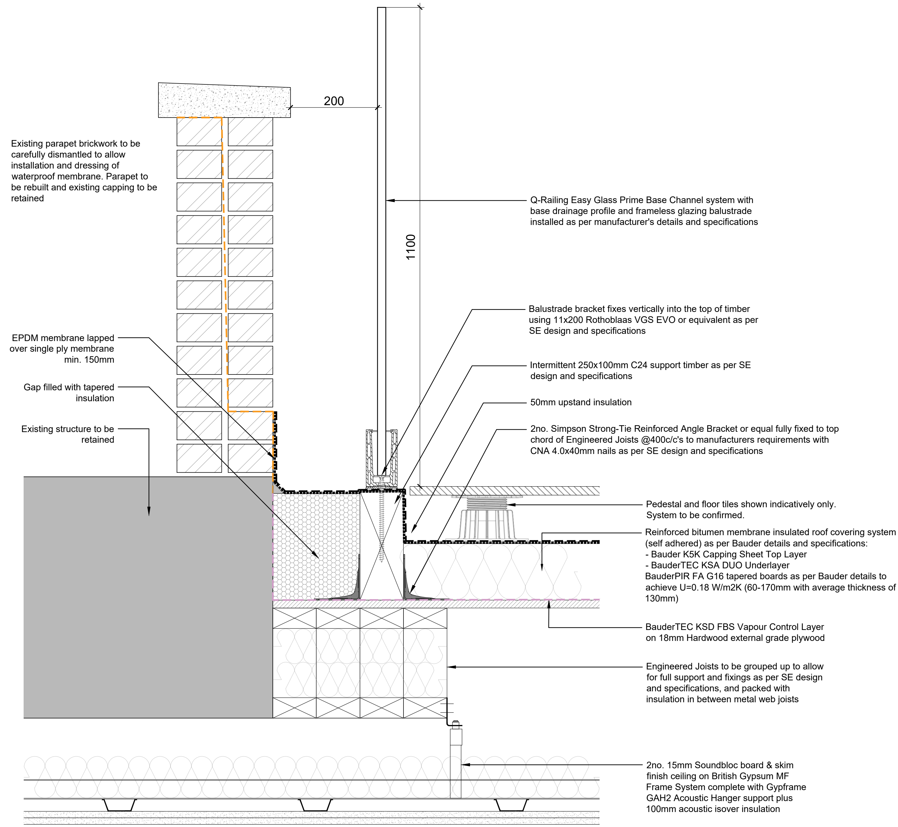
1 Glazed Balustrade Detail 1:5
