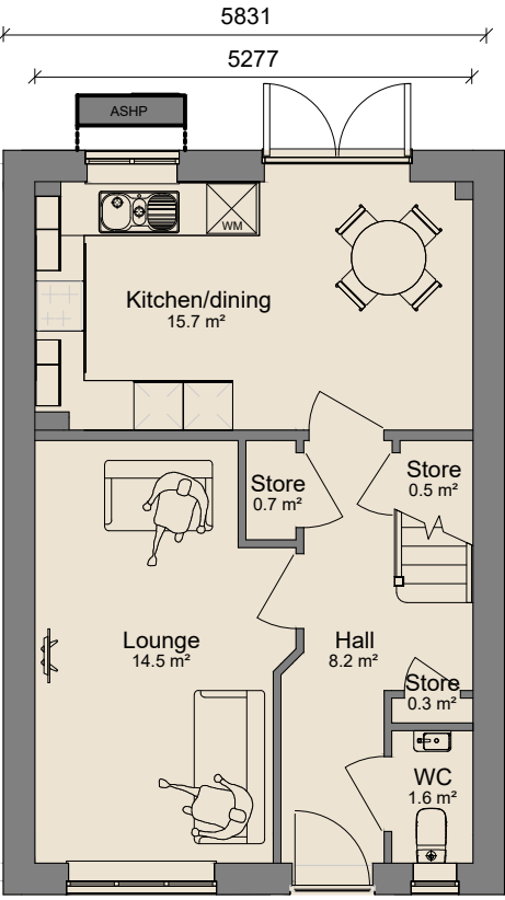
Ground Floor 1 : 100
