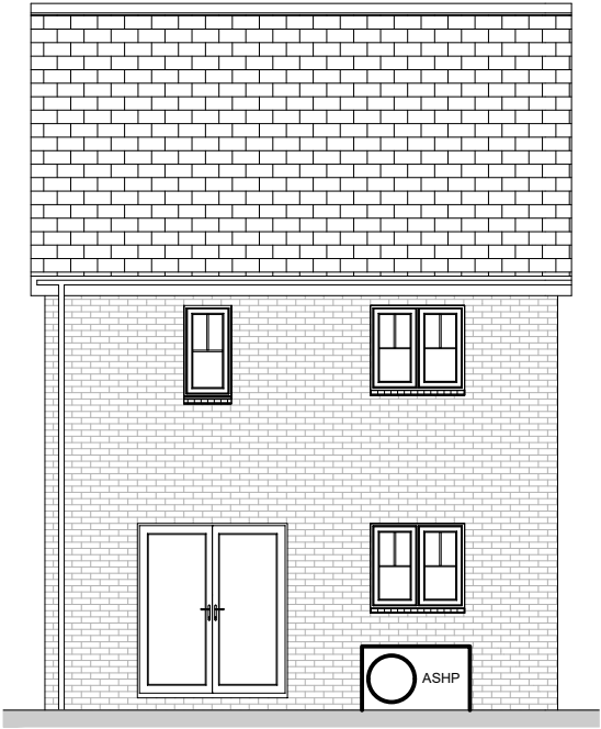
Rear Elevation 1 : 100
