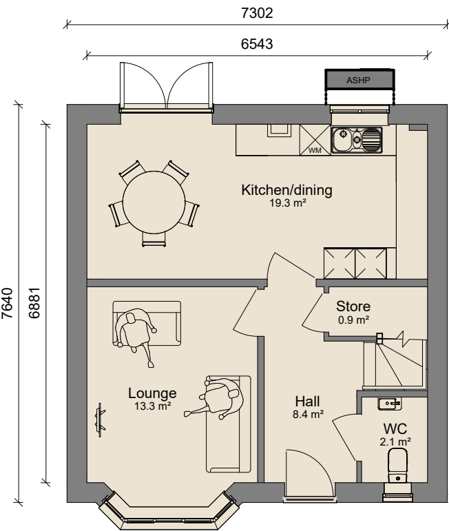
Ground Floor 1 : 100
