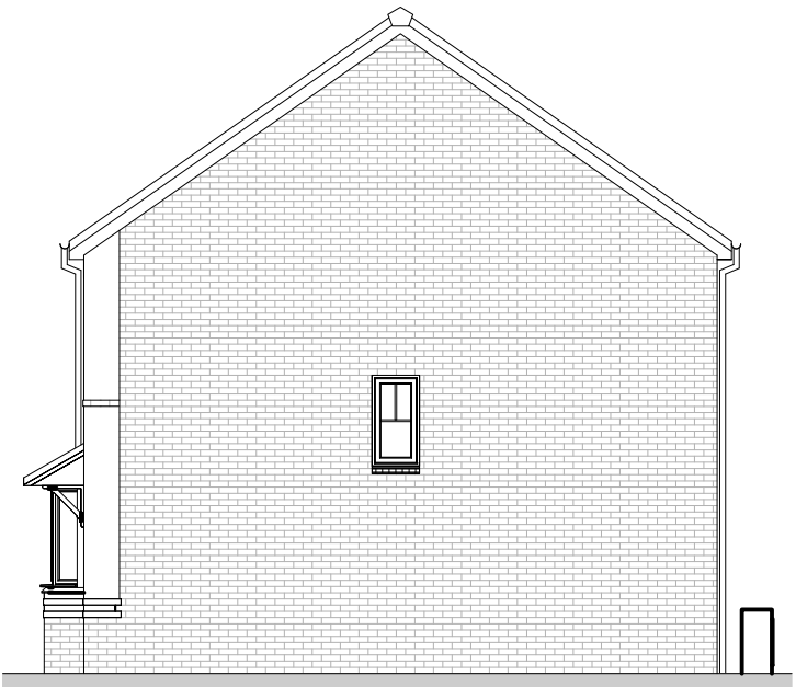
Side Elevation 1 : 100
