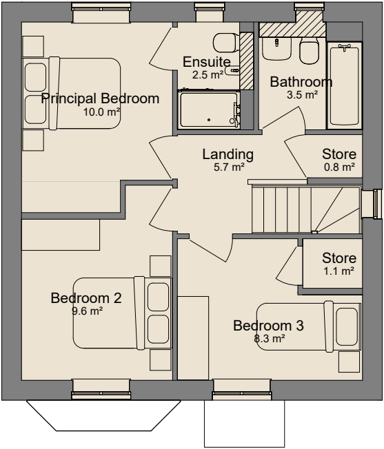
First Floor 1 : 100
