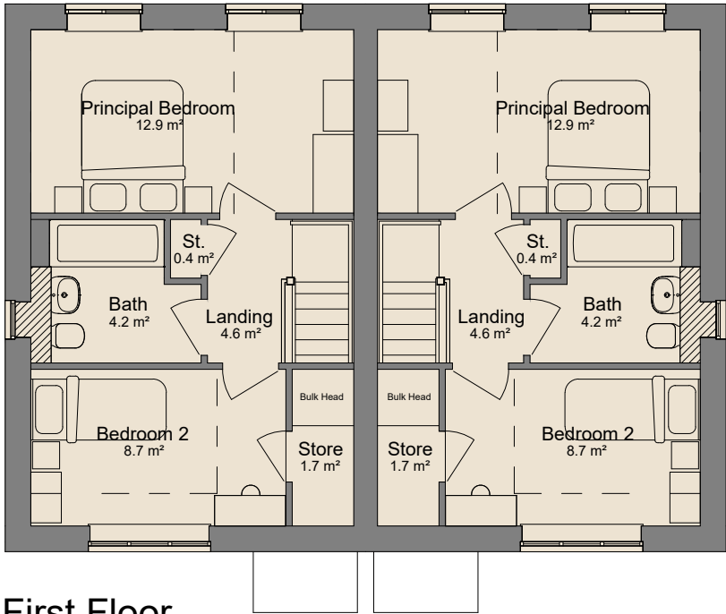
First Floor 1 : 100
