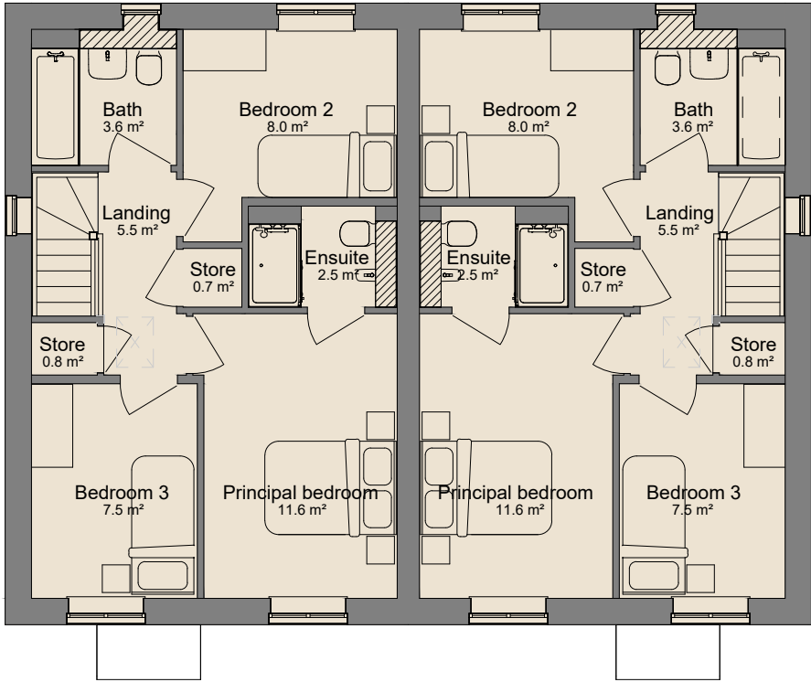
First Floor 1 : 100
