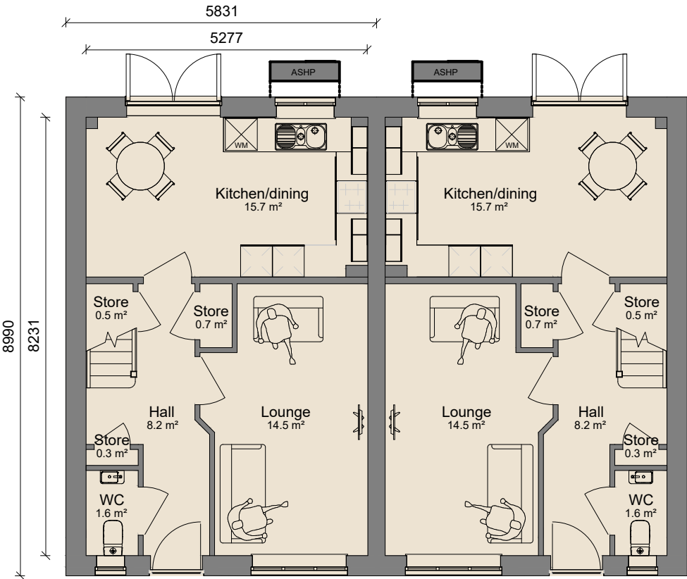
Ground Floor 1 : 100
