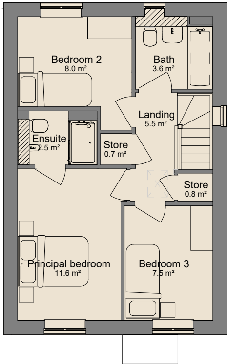
First Floor 1 : 100
