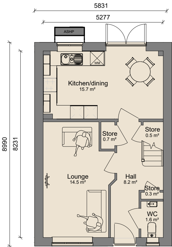
Ground Floor 1 : 100
