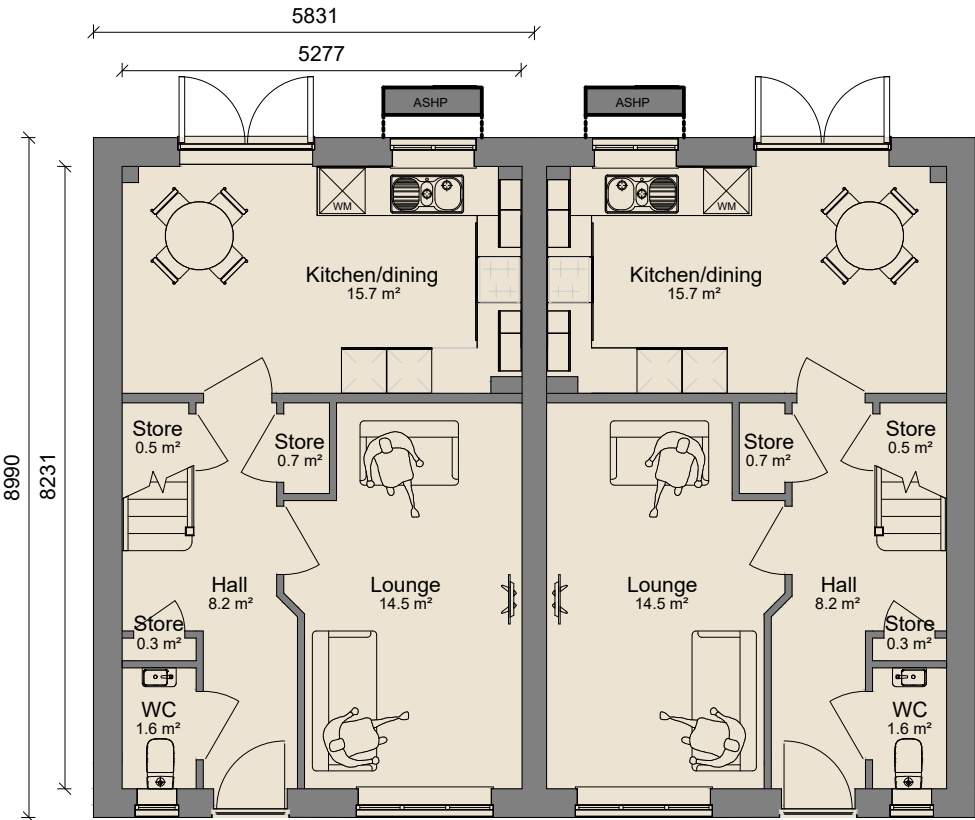
Ground Floor 1 : 100
