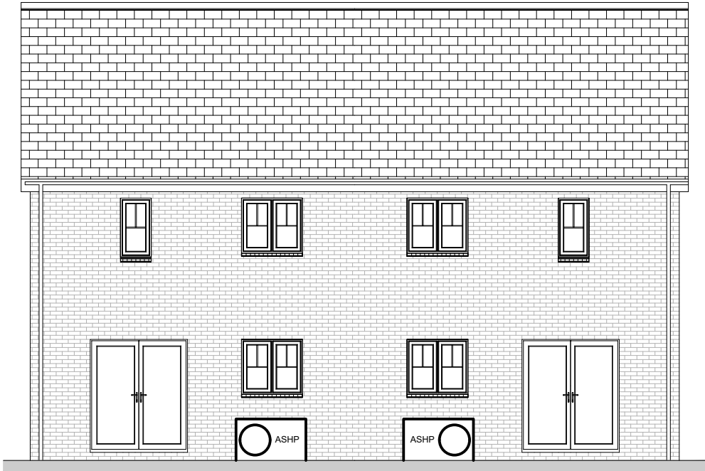
Rear Elevation 1 : 100
