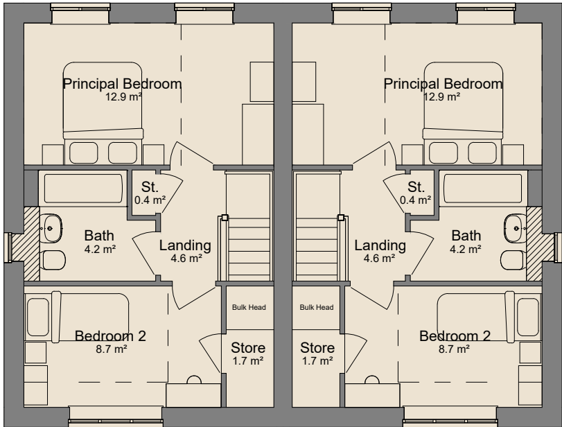
First Floor 1 : 100
