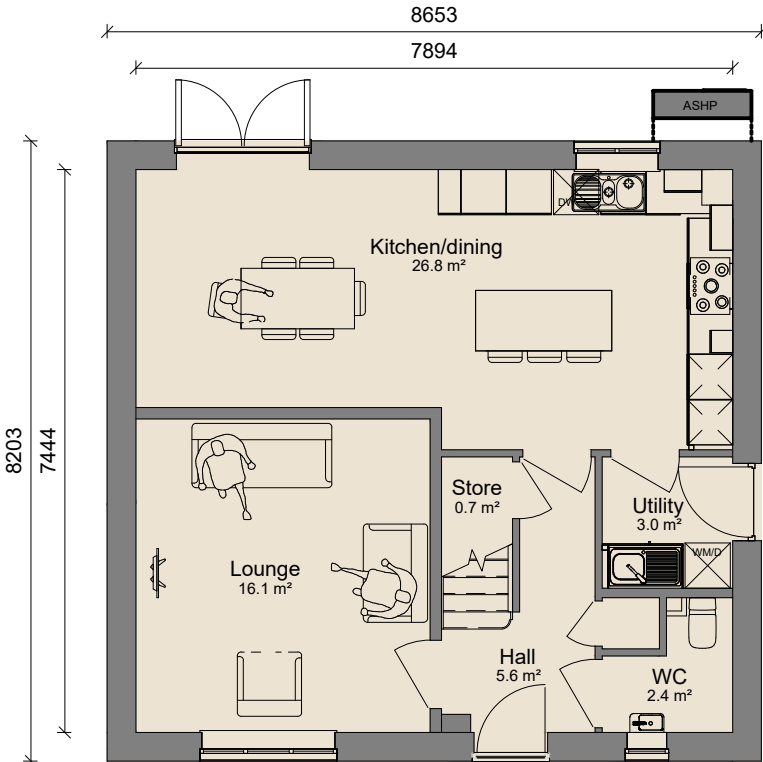
Ground Floor 1 : 100
