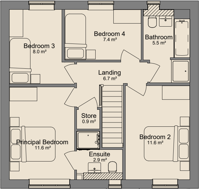
First Floor 1 : 100
