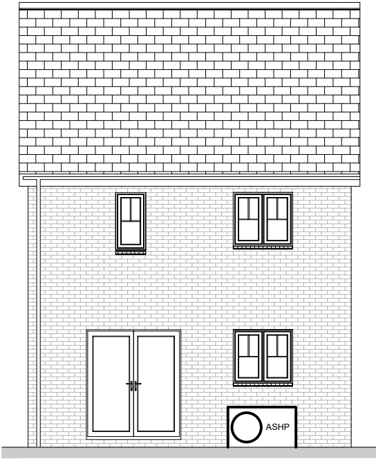
Rear Elevation 1 : 100
