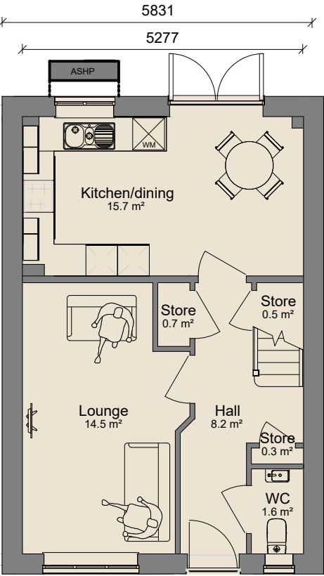
Ground Floor 1 : 100
