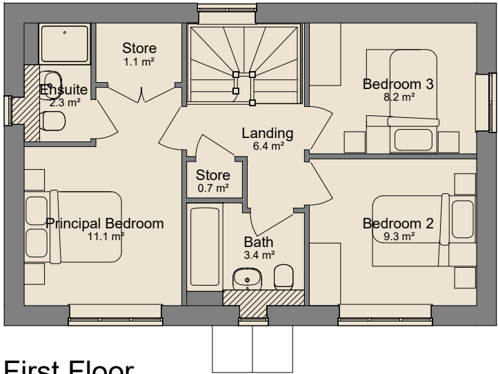
First Floor 1 : 100
