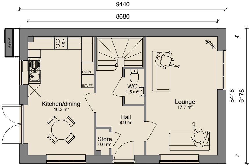
Ground Floor 1 : 100
