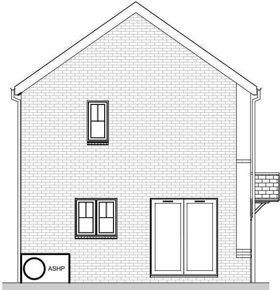
Side Elevation 1 : 100
