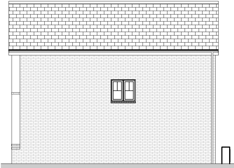
Rear Elevation 1 : 100
