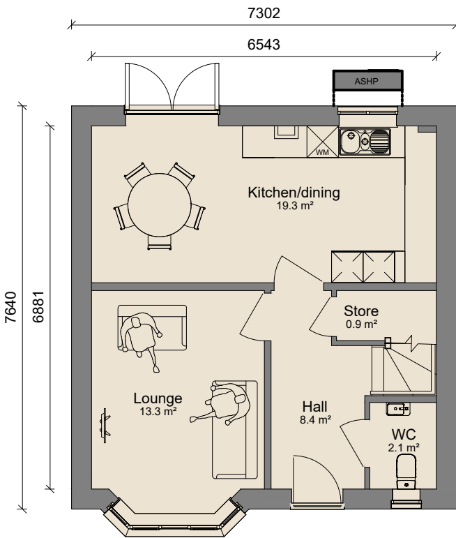
Ground Floor 1 : 100
