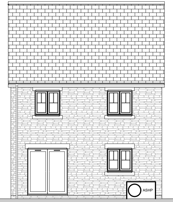
Rear Elevation
