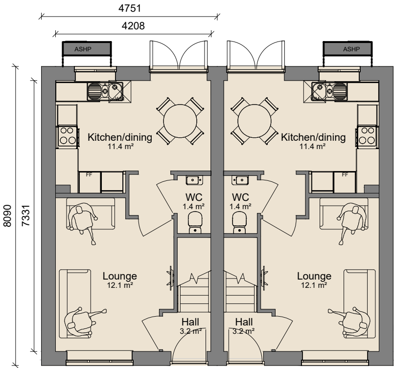
Ground Floor 1 : 100
