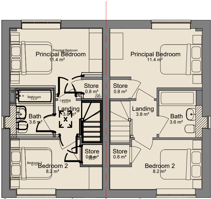
First Floor 1 : 100
