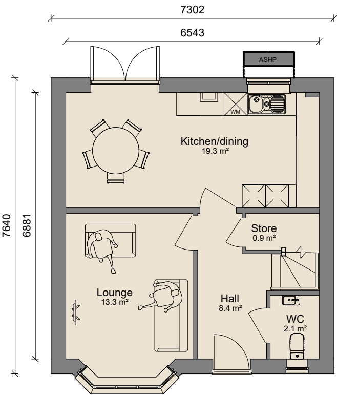
Ground Floor 1 : 100
