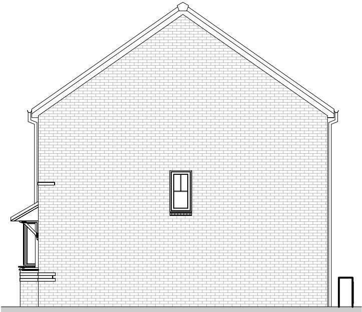
Side Elevation 1 : 100
