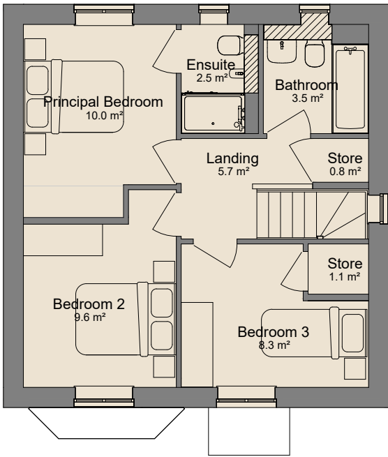
First Floor 1 : 100
