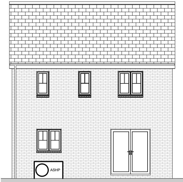
Rear Elevation 1 : 100
