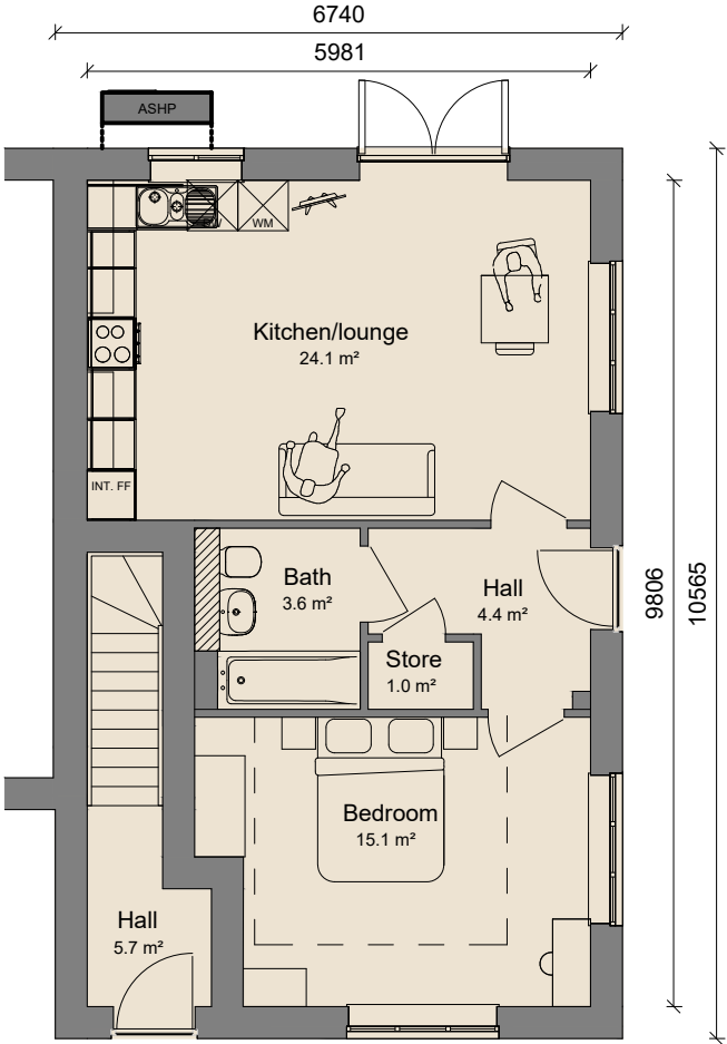
Ground Floor 1 : 100
