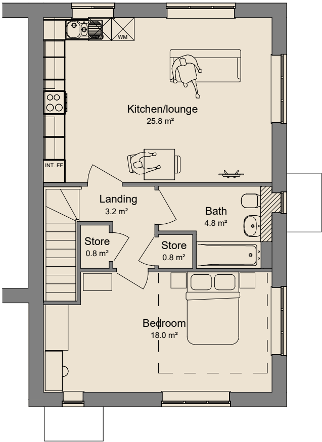
First Floor 1 : 100
