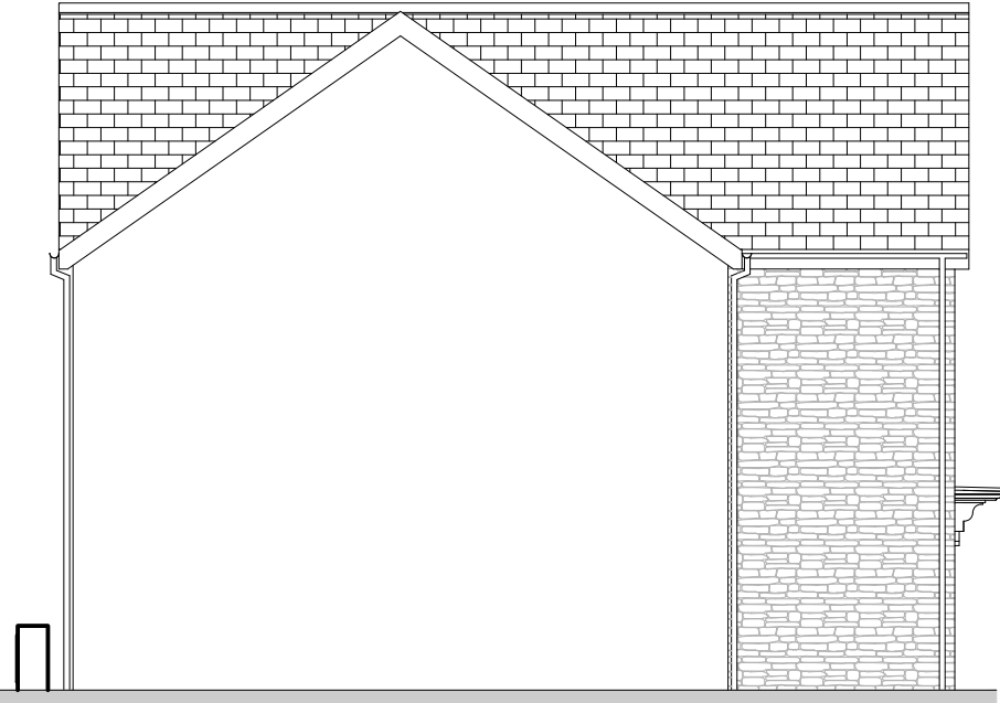
Rear Elevation 1 : 100
