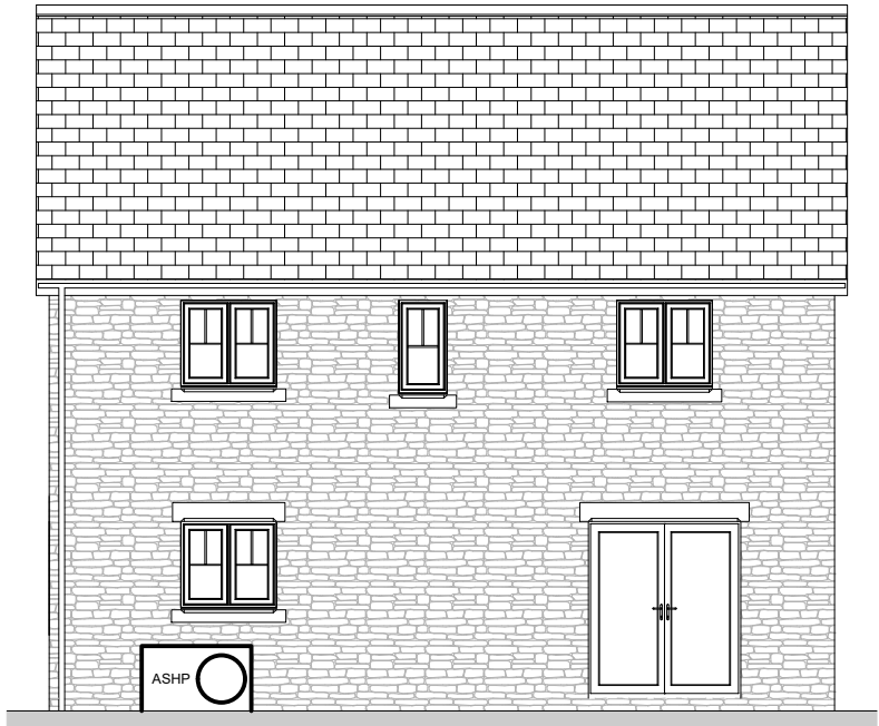
Rear Elevation 1 : 100
