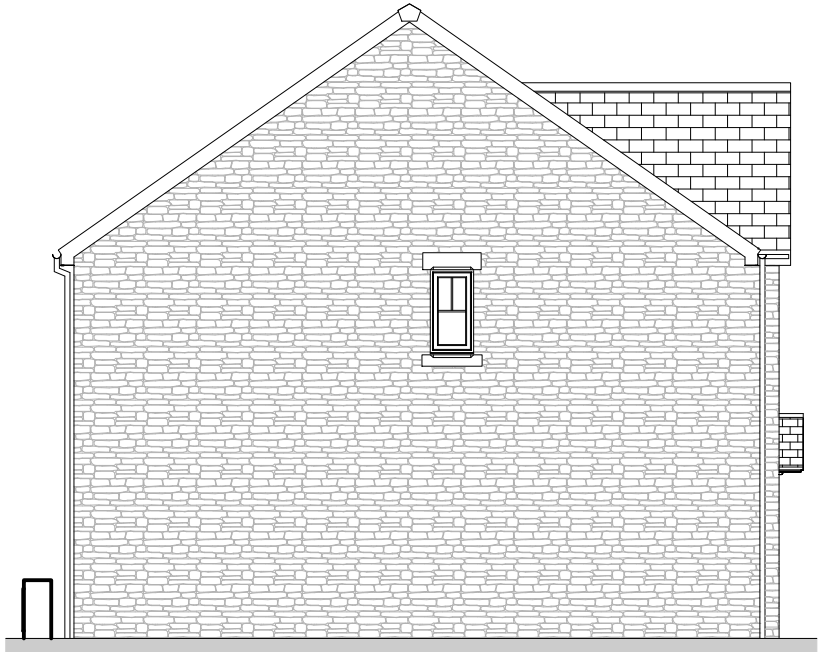
Side Elevation 1 : 100
