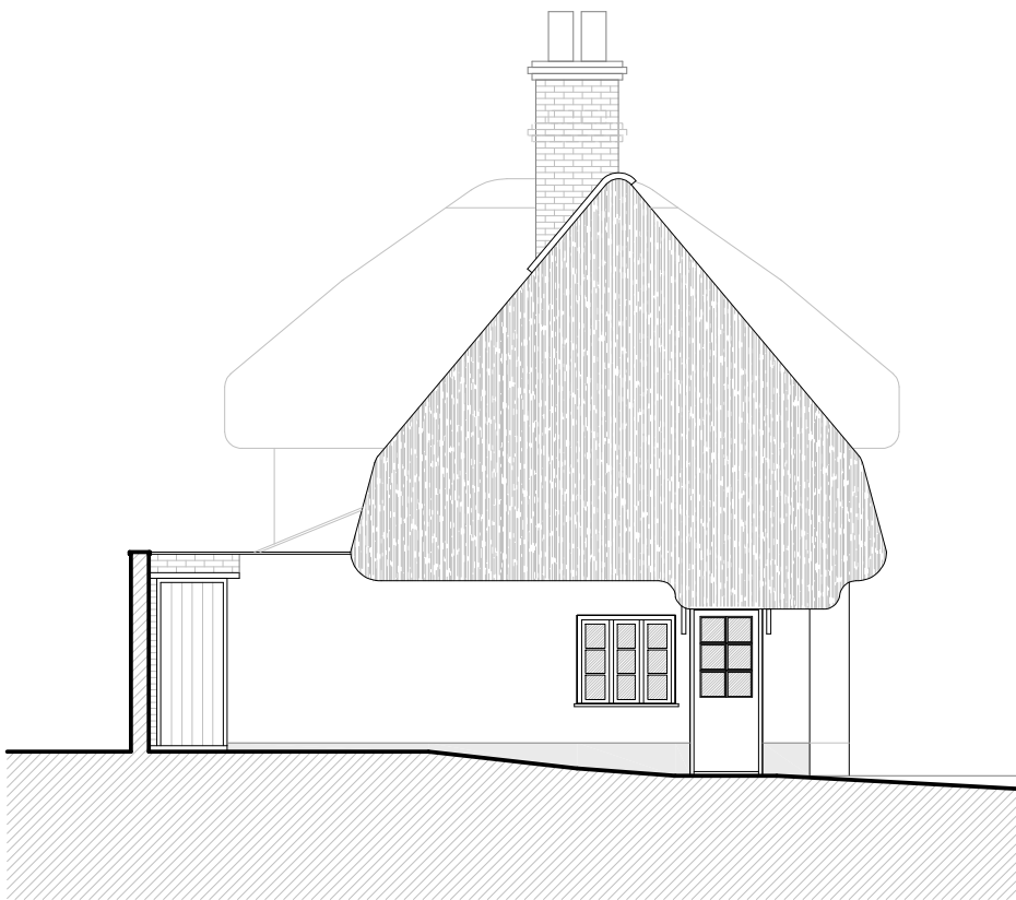
North Elevation
