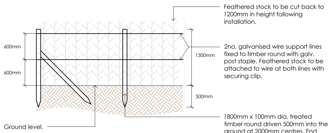
Detail 10 - Typical Feathered Stock Support Detail (N.T.S.)
