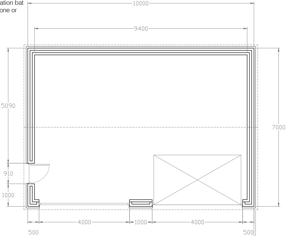
Floor Plan
