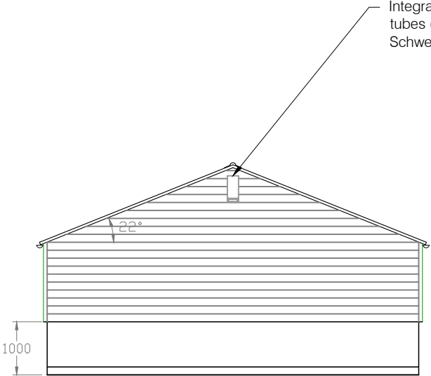
South Elevation
