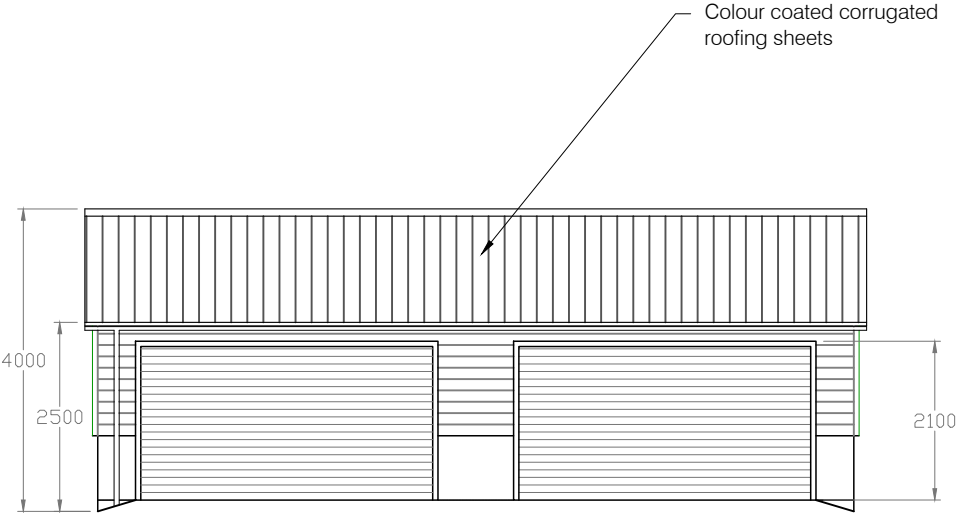
West Elevation
