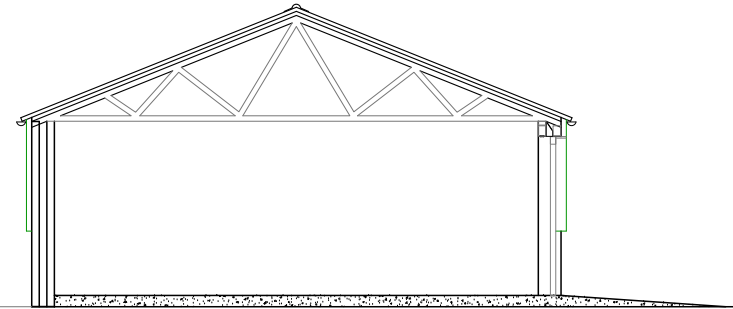
Cross Section
