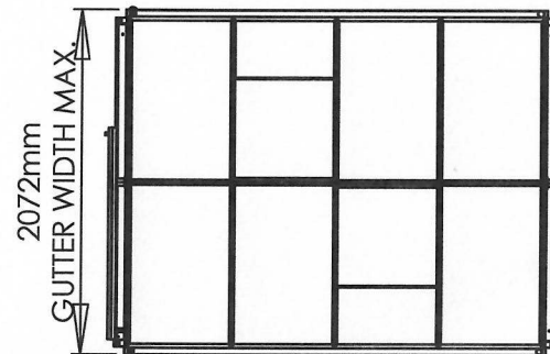
ROOF PLAN
