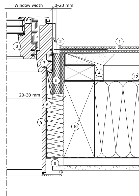
Section B-B 1:5
