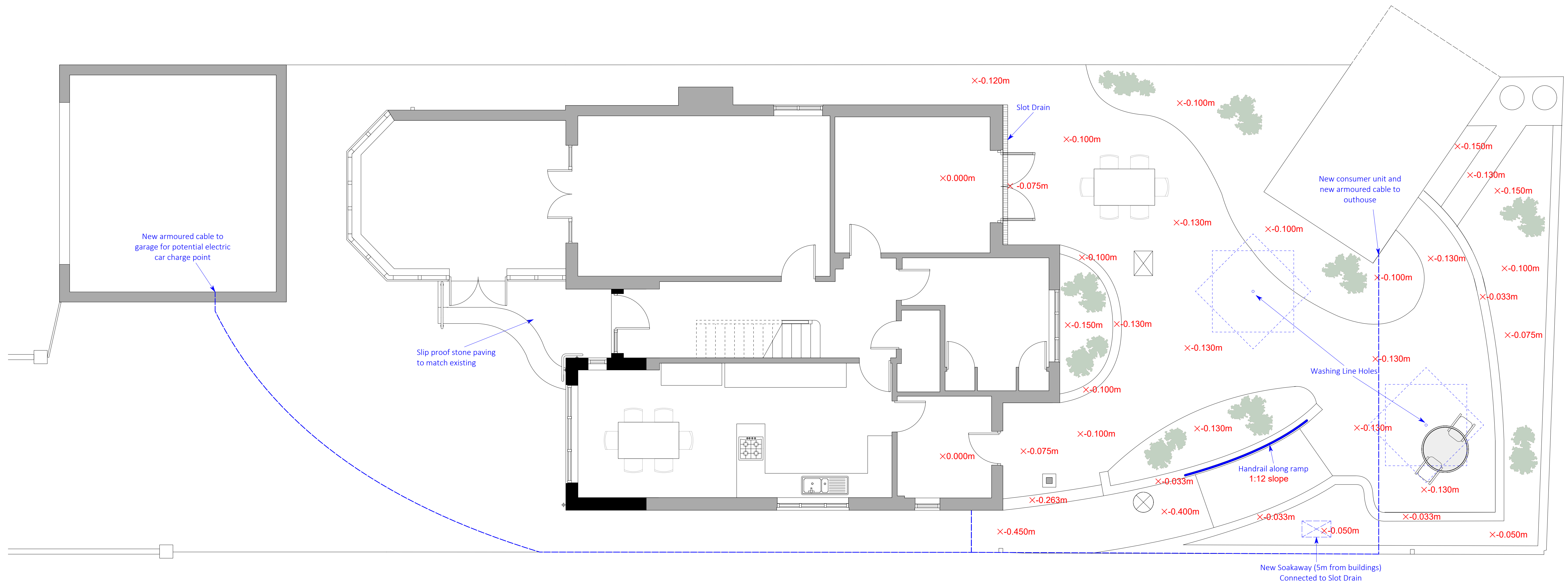
PLN 01 Proposed Garden Plan 1:50
