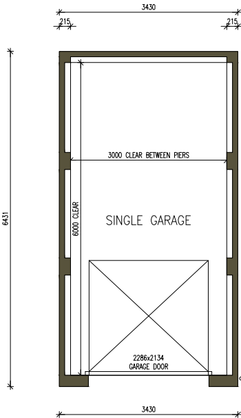
Plan
