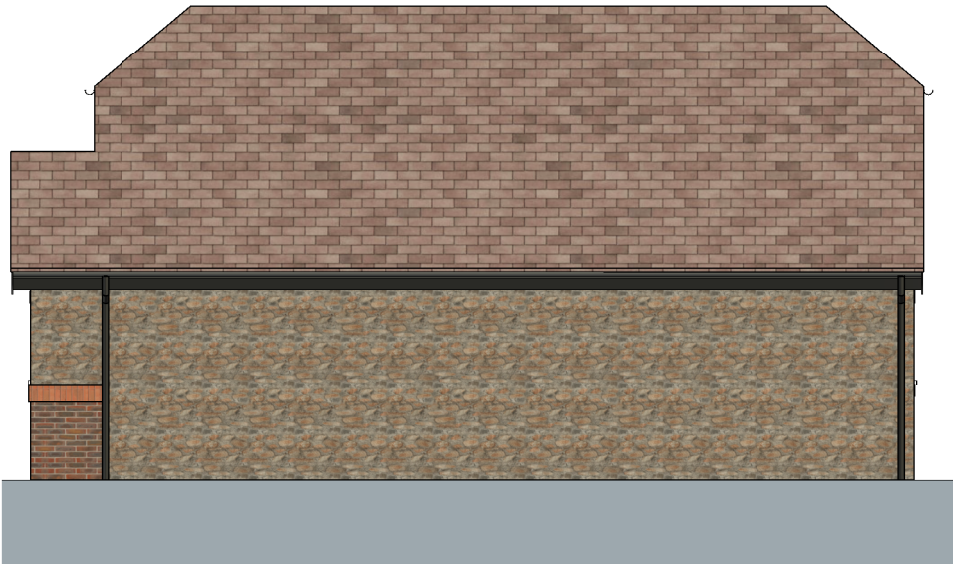
Side Elevation 1 : 100
