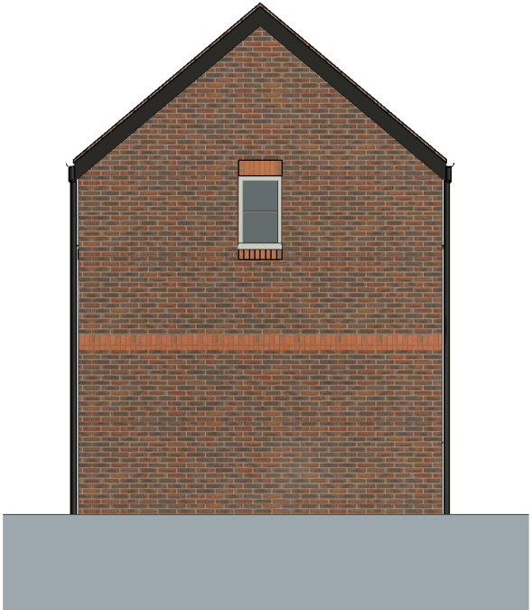
Side Elevation 1 : 100
