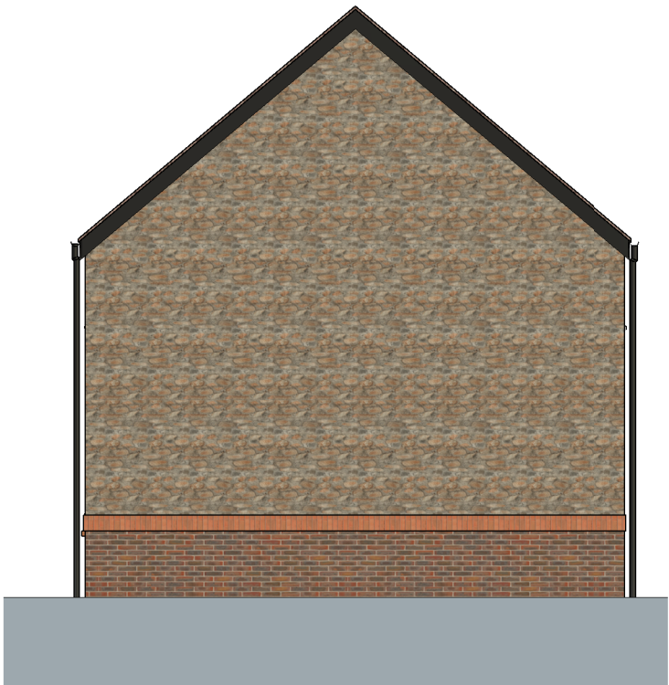
Side Elevation 1 : 100
