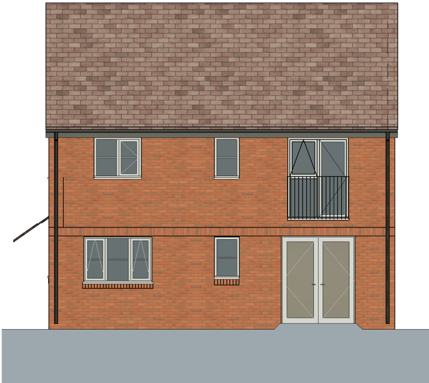
Side Elevation 1 : 100
